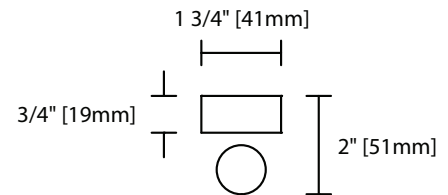
ST-RM Cross Section View
