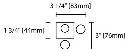
ST2-SM Cross Section View
