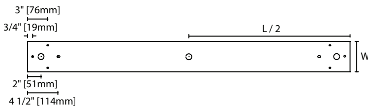
ST-SM Base View
