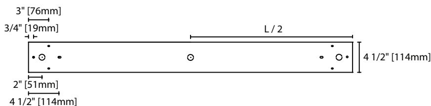
CLB Base View
