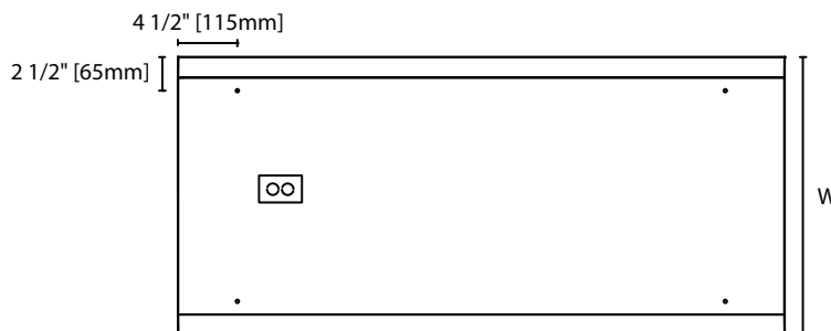
HBD 6/8 Base View
