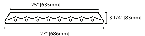
HBD 8 Lamps Cross Section View
