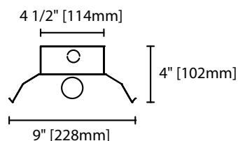
HO1 R Cross Section View
