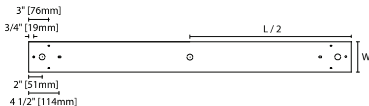
HO1 R Base View
