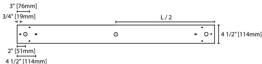
ST3 R Base View
