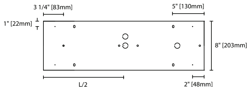
VN Base View
