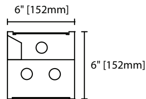
CBB 1UP2D Cross Section View
