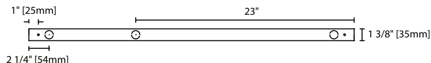
SM1 T5 Base View
