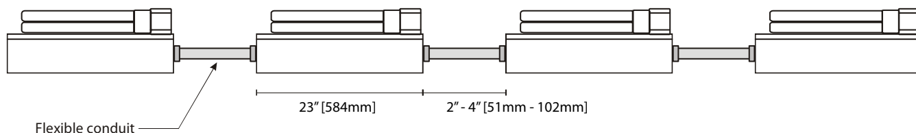
ST-CF Side View
