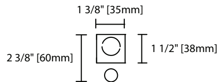
ST1 T5 Cross Section View
